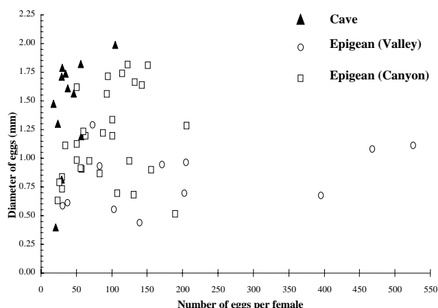
Figure 5. Relationships between eggs diameter and fecundity in 53 mature females from different habitat rivers: subterranean rivers, canyon and valley
