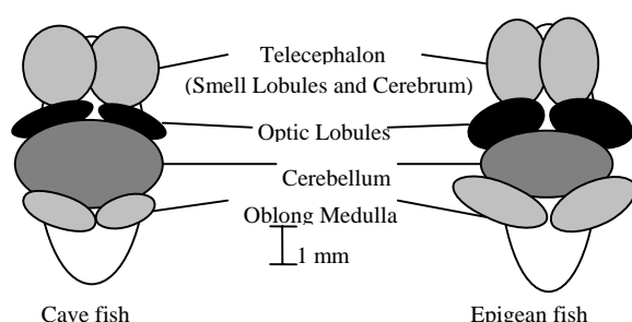
Figure 4. Comparison scheme of encephalon of epigeal and hypogean Trichomycterus (based on surface calculation of each parts of the encephalon in 30 individuals)
